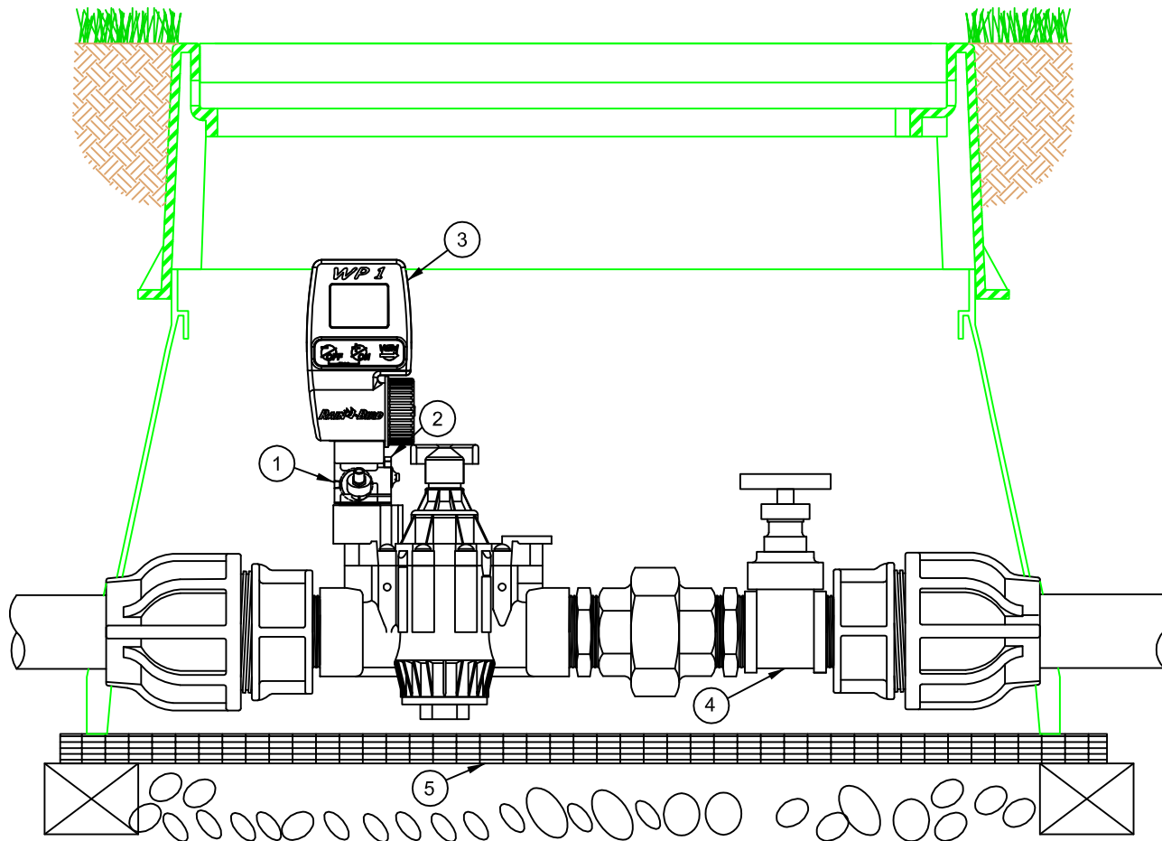
VALVOLA PGA + PRS-DIAL/WP1
